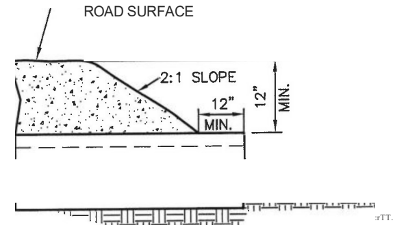
CULVERT DETAIL
